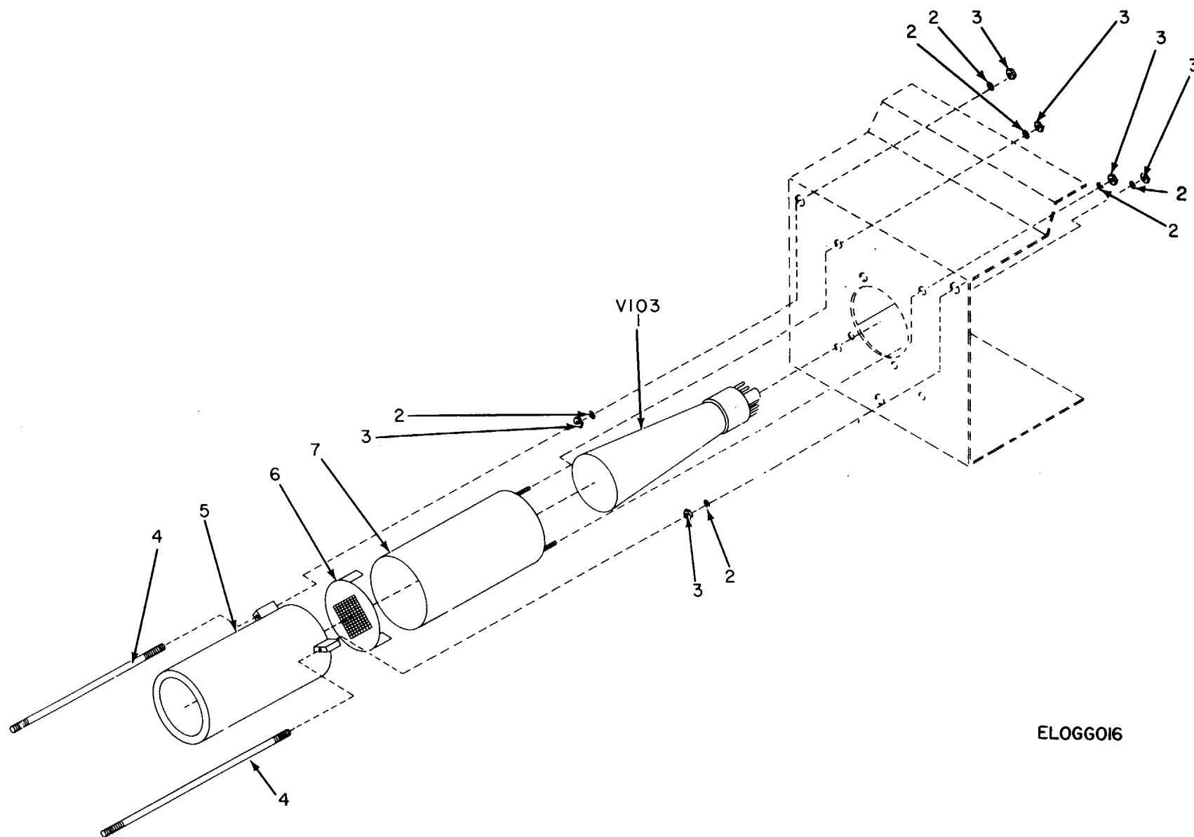
Figure 8. Generator, Signal TS-452E/U, CRT Light Shield Assembly.
