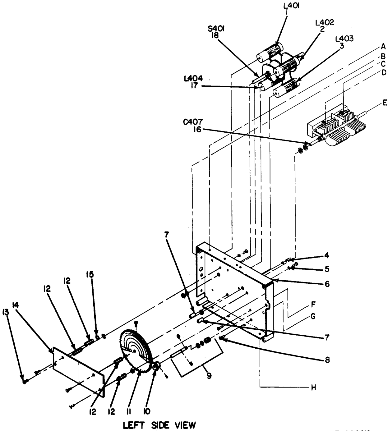
Figure 4. Generator, Signal TS-452E/U, Wavemeter (Sheet 1 of 3).
