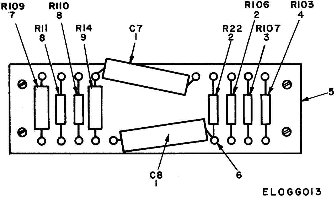
Figure 5. Generator, Signal TS-452E/U, Electronic Component Assembly No. 1.
