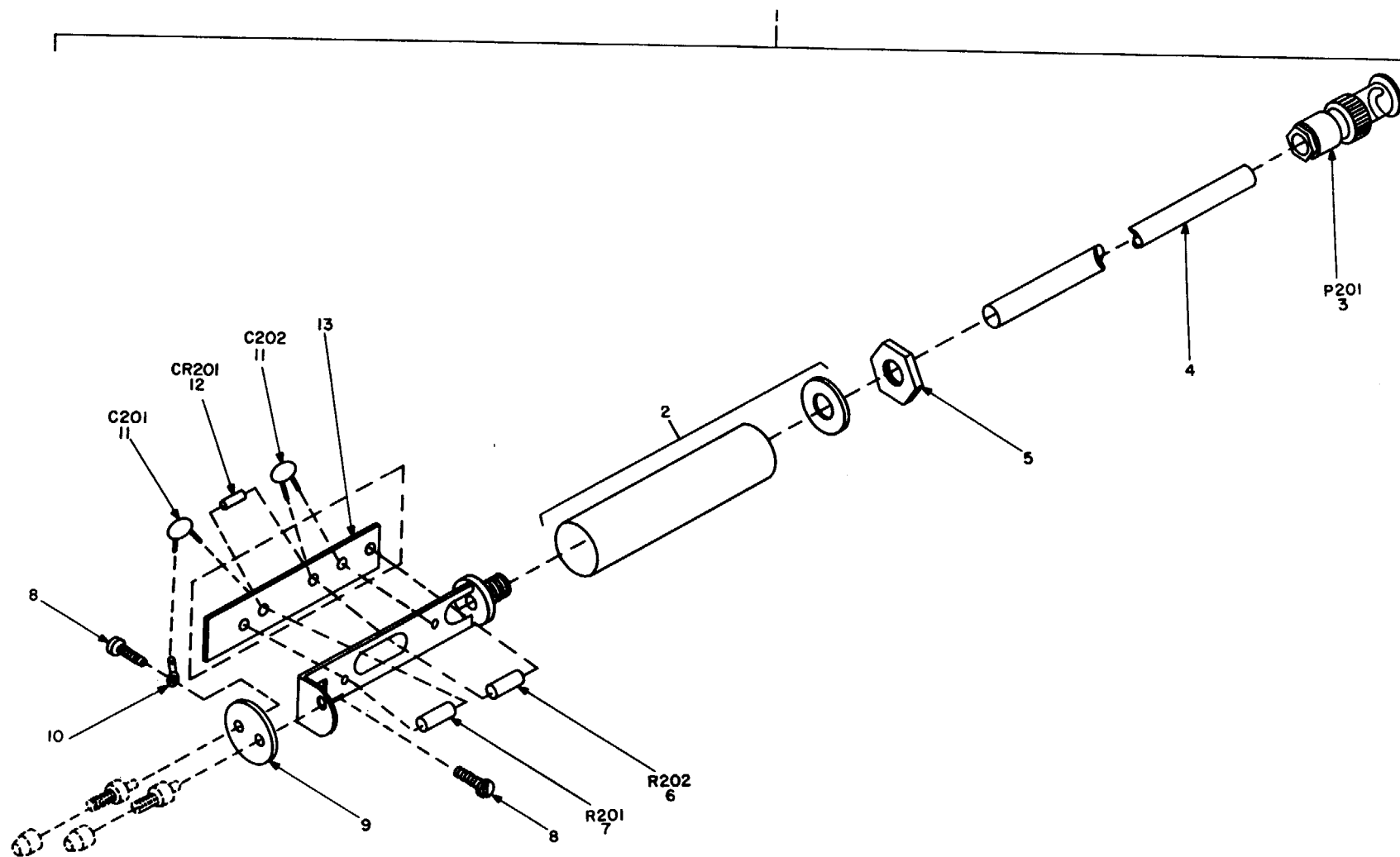
Figure 9. Generator, Signal TS-452E/U, Detector, Radio Frequency.
