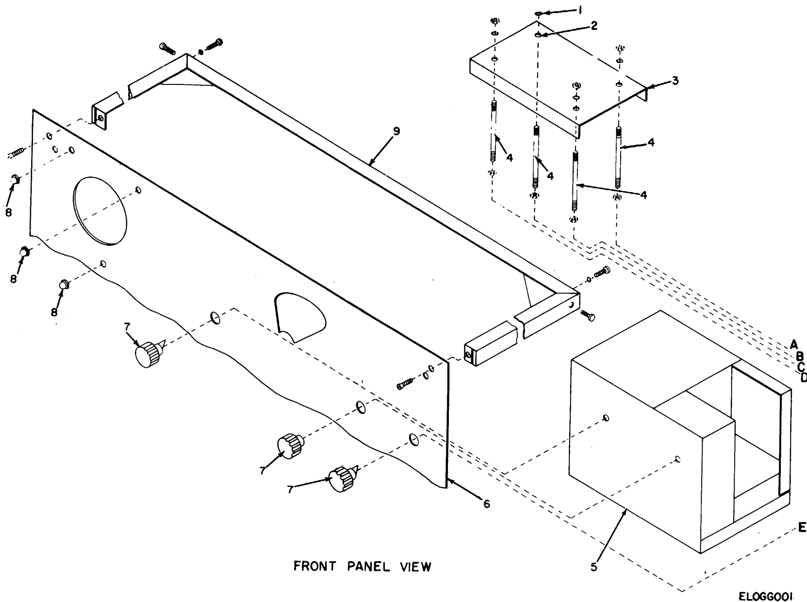
Figure 1. Generator, Signal TS-452E/U (Sheet 1 of 3).
