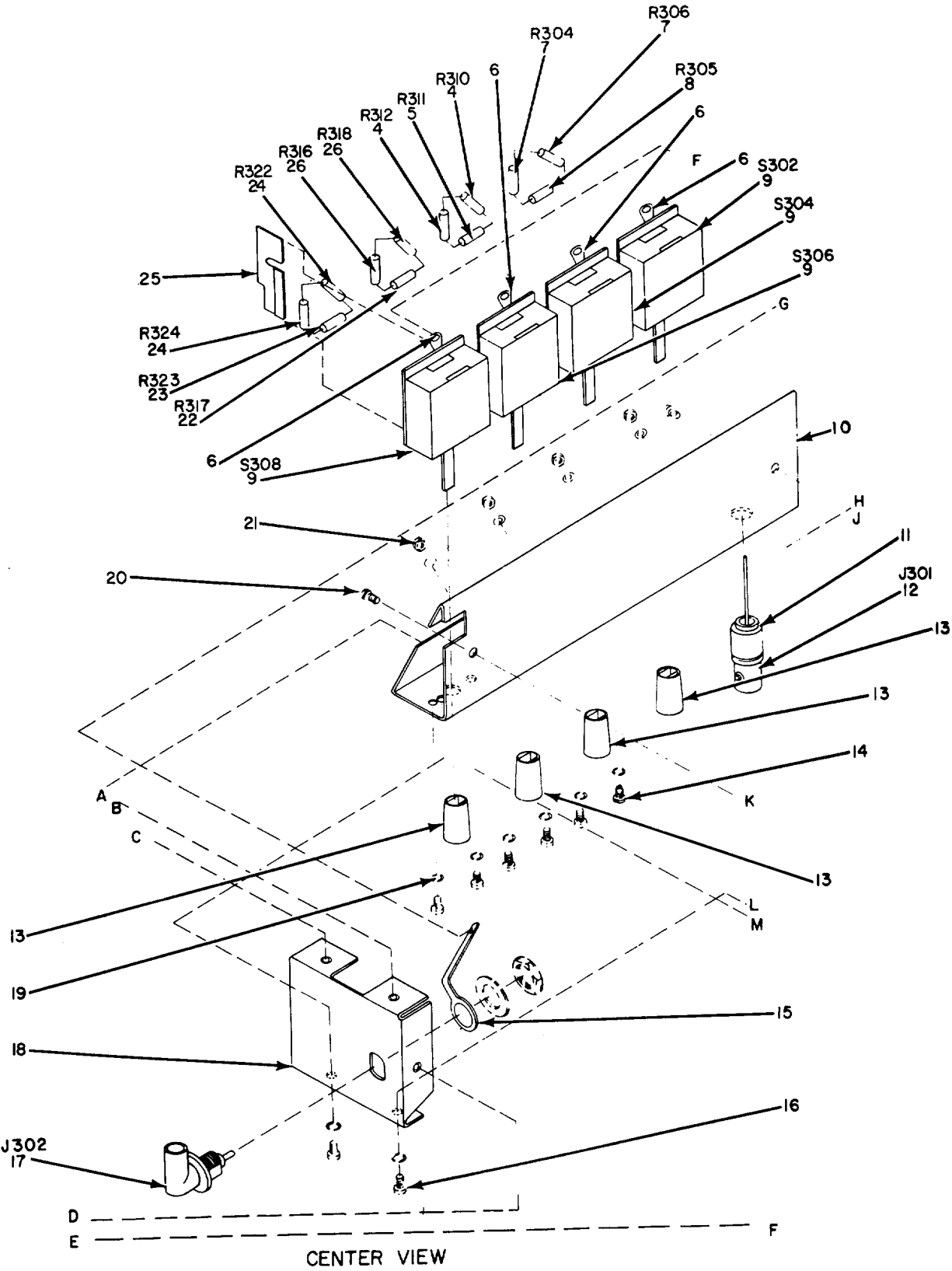
Figure 3. Generator, Signal TS-452E/U, Attenuator, Variable (Sheet 2 of 3).
