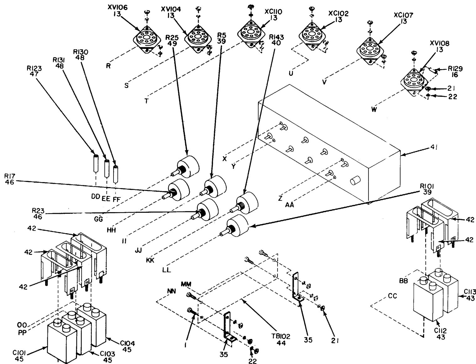
BOTTOM VIEW, ATTENUATOR COMPONENTS
