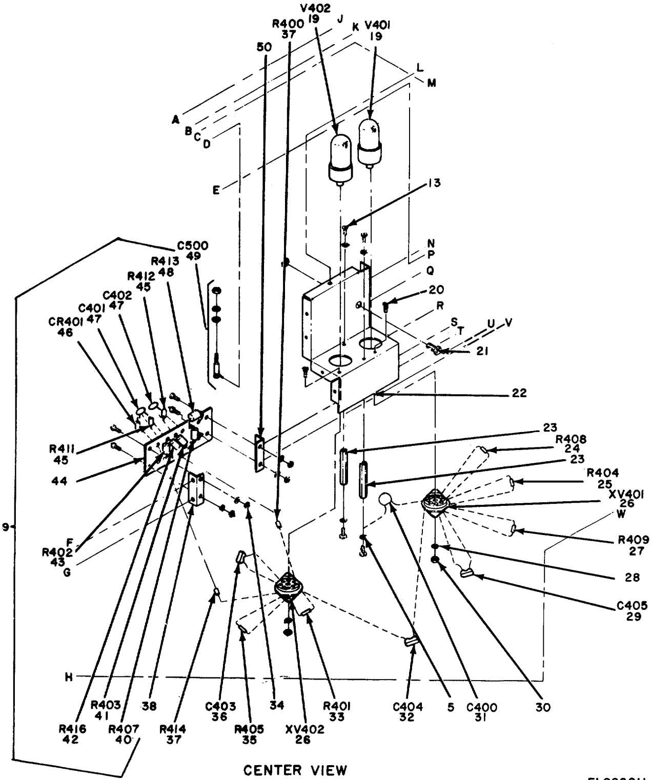
Figure 4. Generator, Signal TS-452E/U, Wavemeter (Sheet 2 of 3).
