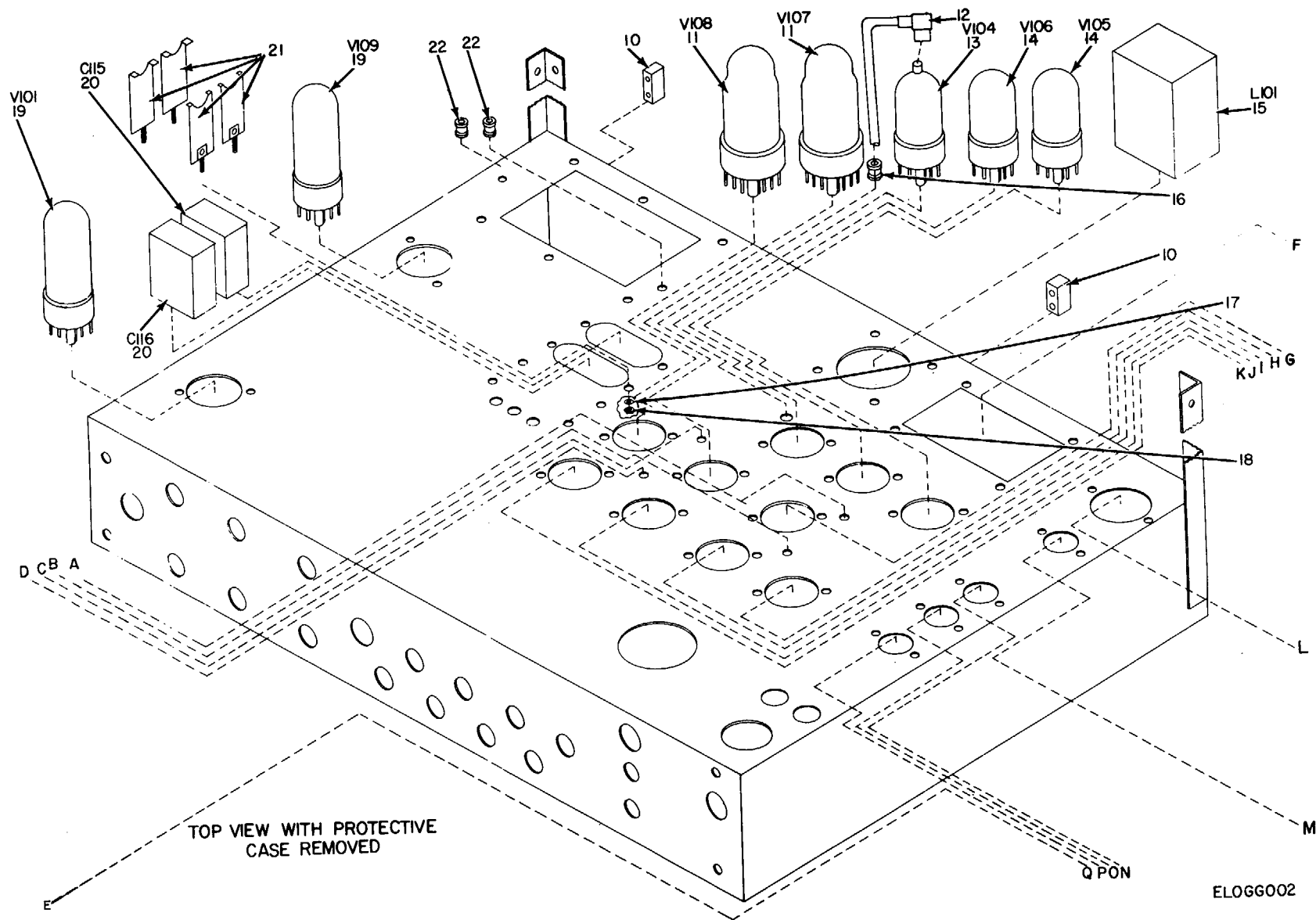
Figure 1. Generator, Signal TS-452E/U (Sheet 2 of 3).
