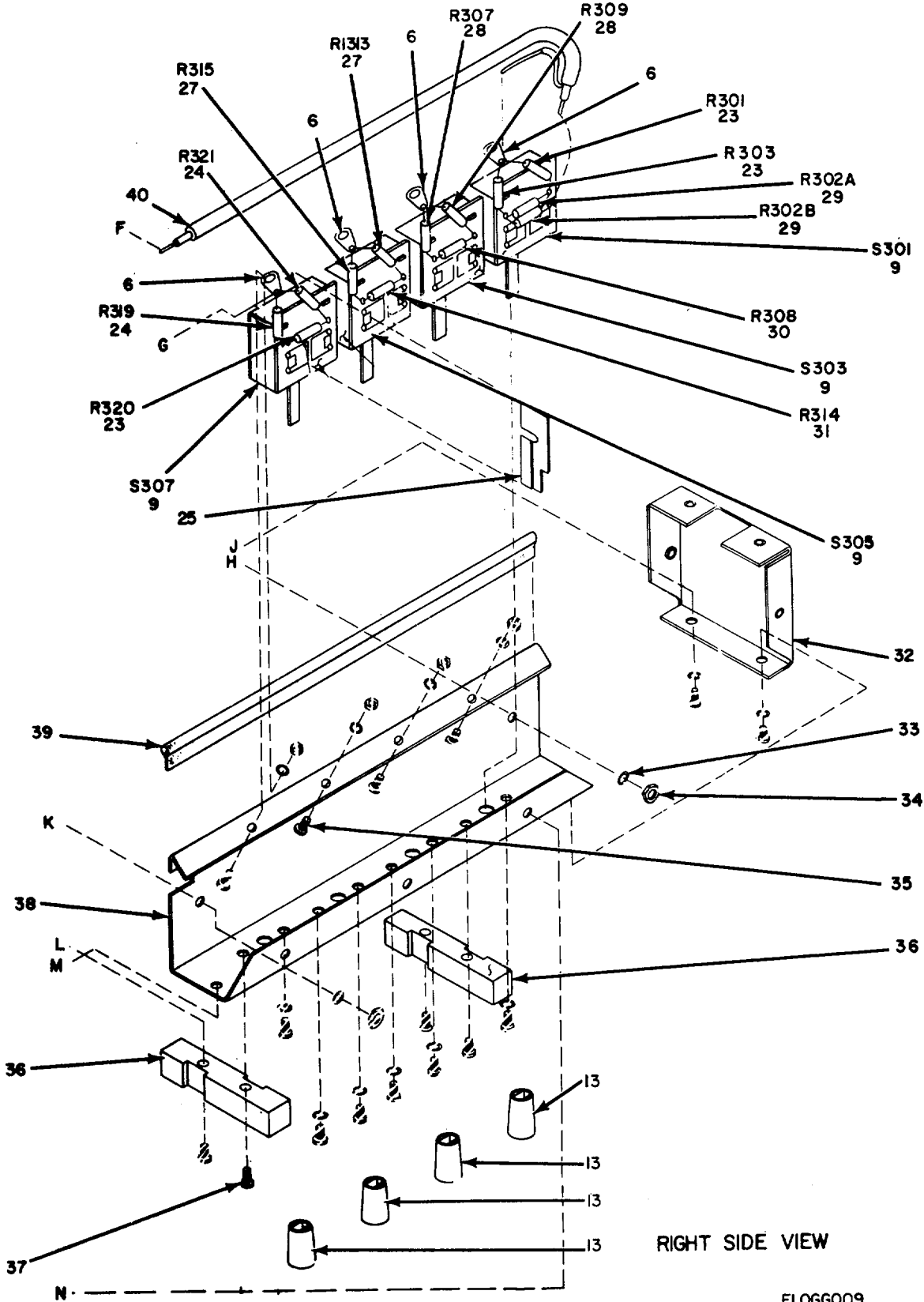
Figure 3. Generator, Signal TS-452E/U, Attenuator, Variable (Sheet 3 of 3).
