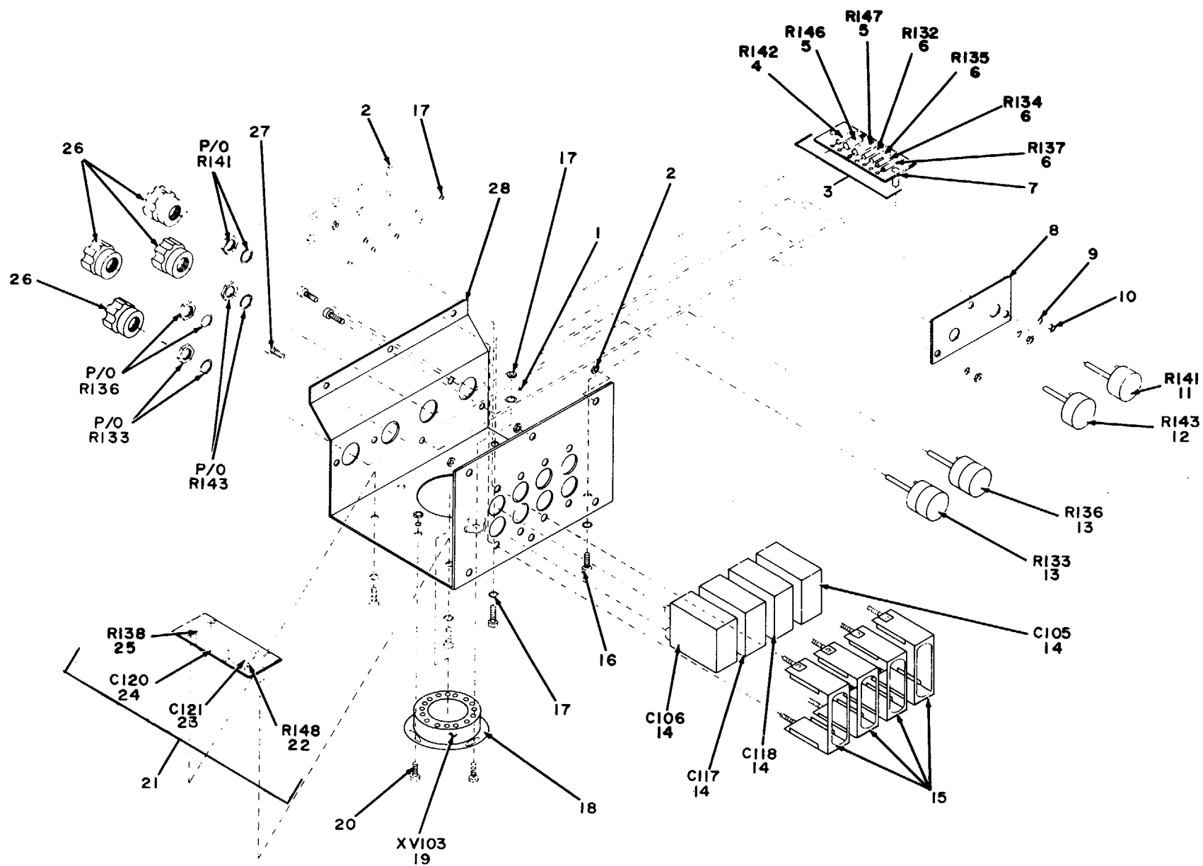
Figure 7. Generator, Signal TS-452E/U, Video Chassis Assembly.
