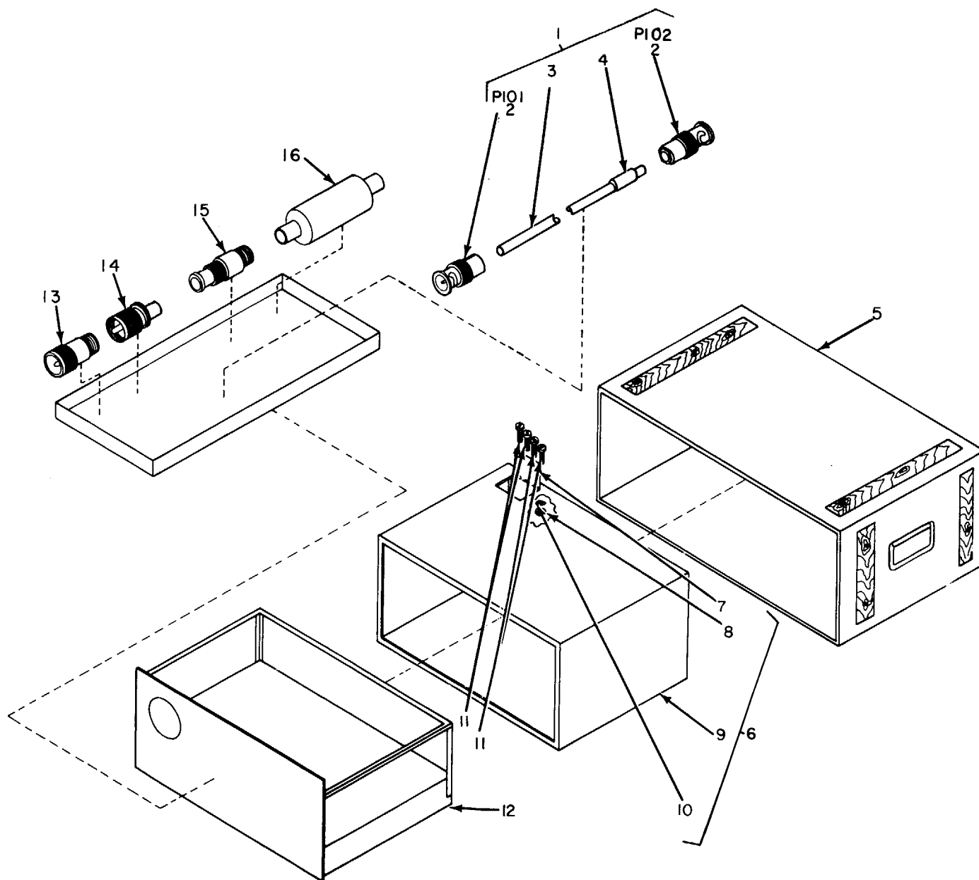
Figure 10. Generator, Signal TS-452E/U, Signal Generator Assembly.
