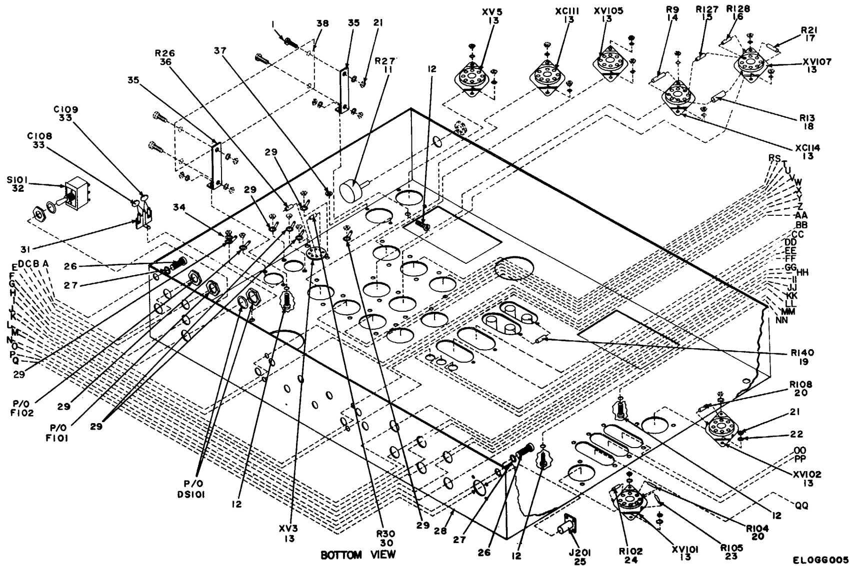
Figure 2. Generator, Signal TS-452E/U, Chassis (Sheet 2 of 3).
