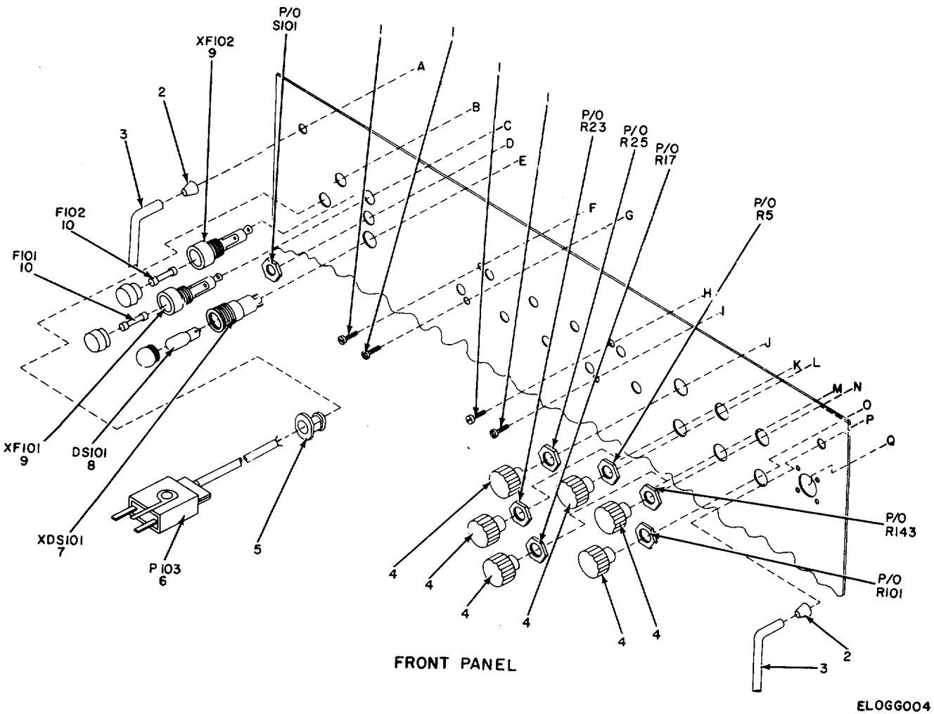
Figure 2. Generator, Signal TS-452E/U, Chassis (Sheet 1 of 3).
