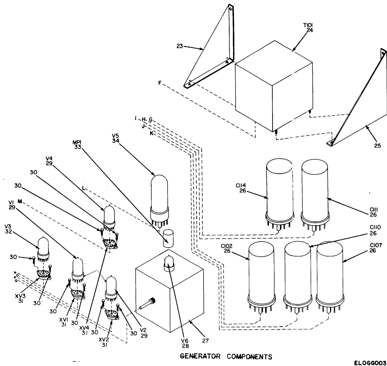
Figure 1. Generator, Signal TS-452E/U (Sheet 3 of 3).
