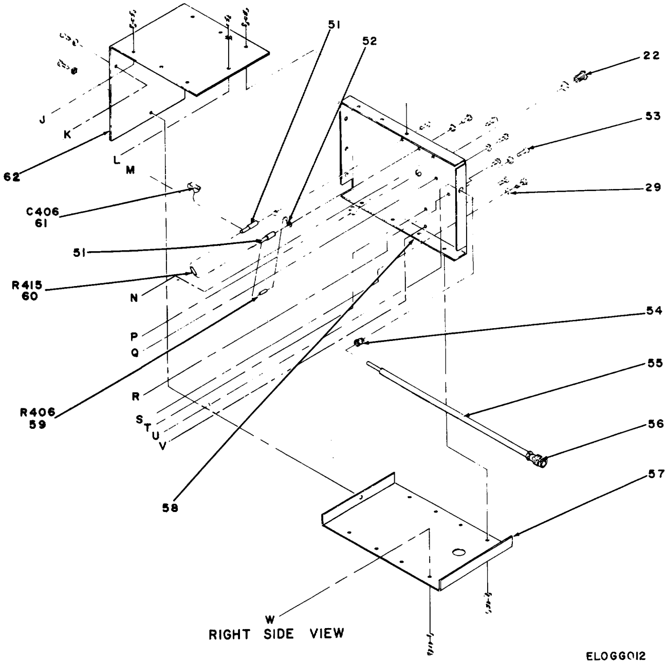
Figure 4. Generator, Signal TS-452E/U, Wavemeter (Sheet 3 of 3).
